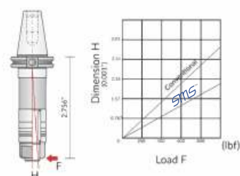
Deflection of a CAT40 holder Conventional vs. AccuPlus
